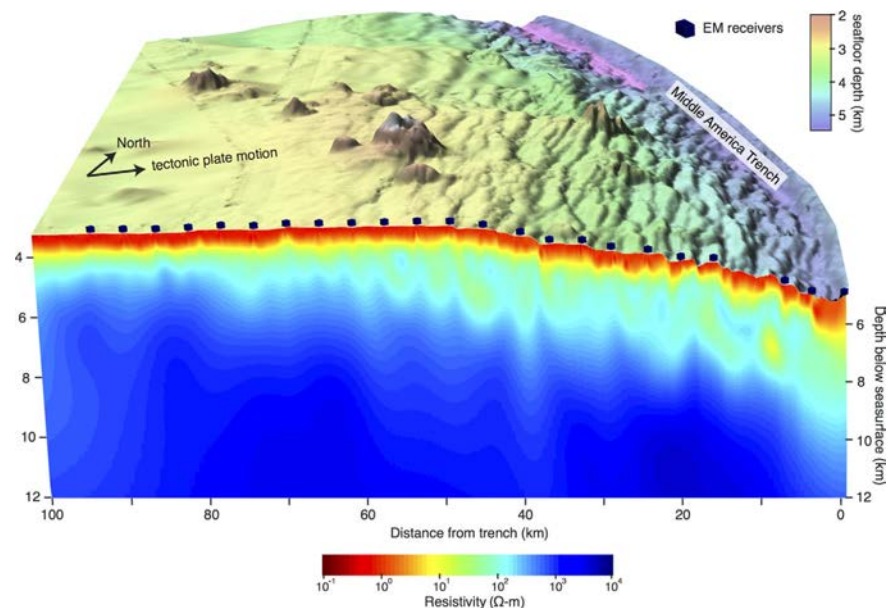
Figure 4. The electrical structure of the incoming Cocos plate from nonlinear inversion of deep-towed CSEM data. The vertical cross section shows the electrical resistivity structure and the stitched top plot shows seafloor bathymetry. The dark blue cubes show the location of EM receivers. The region of the seafloor marked by steeply dipping bathymetric relief correlates with subvertical conductive channels, which we interpret as evidence for the migration of seawater along bending faults.
